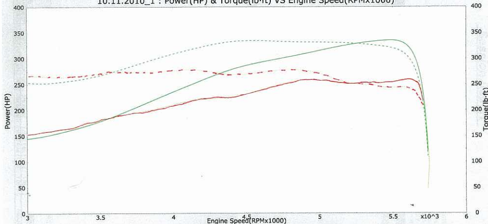
10.11.2010_1 : Power(HP) & Torque(lb-ft) VS Engine Speed(RPMx1000)
